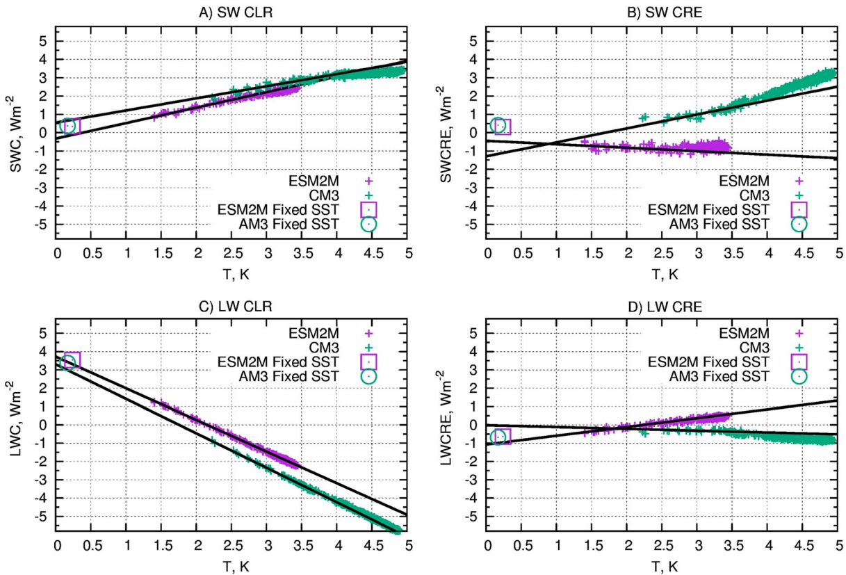
Figure 2. Individual components of N plotted against T for the 2XS runs. The 2\times\text{CO}_2 fixed SST runs are also shown. Lines indicate the fits calculated by the LE method applied to years 51–350 (~P2).
