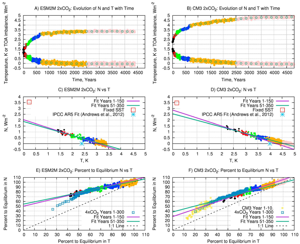
Figure 1. T and N (each filled circle is a 5 year average and clear circle a 200 year average) for years since \text{CO}_2 is fixed in the 2XS experiments of ESM2M (a) and CM3 (b). N plotted against T (5 year averages) is shown for ESM2M (years 1–2500) (c) and CM3 (d). The LE method applied to years 1–150 and years 51–350 is shown along with the LE method estimates of ECS from the 4XI experiments published in Andrews et al. (2012) that were used in IPCC-AR5. Percent to equilibrium in N (i.e., N(T = 0 \text{ K}) to N(T = \text{ECS}) ) versus percent to equilibrium in T (i.e., T = 0 to ECS) are plotted for ESM2M (e) and CM3 (f). Color code for 2XS runs in all panels: Period 2: black (years 1–50), red (years 51–150), green (years 151–350). Period 3: blue (years 351–700), orange (years 701 to 2500), pink (years 2501–4800).
