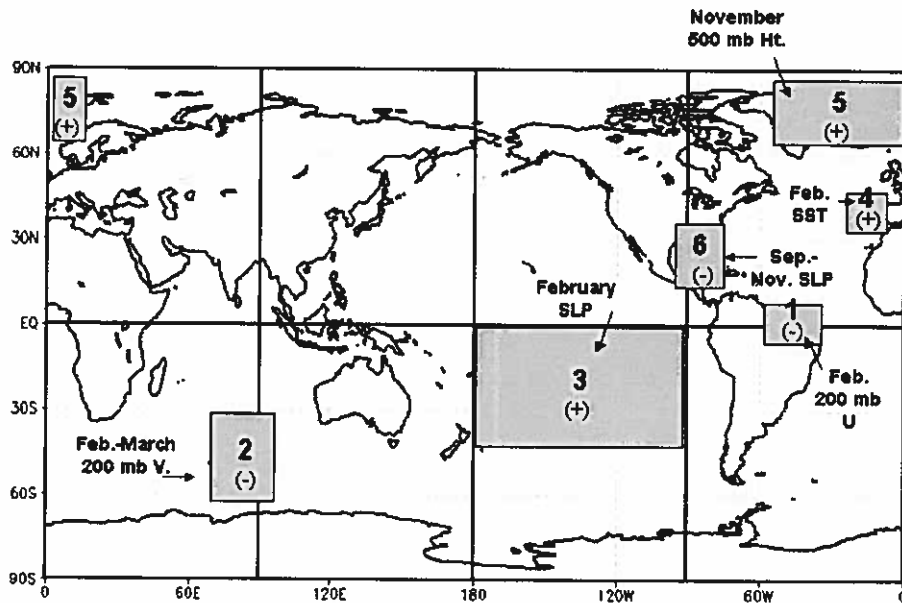
Figure 1: Location of predictors for our early April forecast for the 2005 hurricane season. A plus (+) means that positive values of the parameter indicate increased hurricane activity this year, and a minus (-) means that positive values of the parameter indicate decreased hurricane activity this year.
