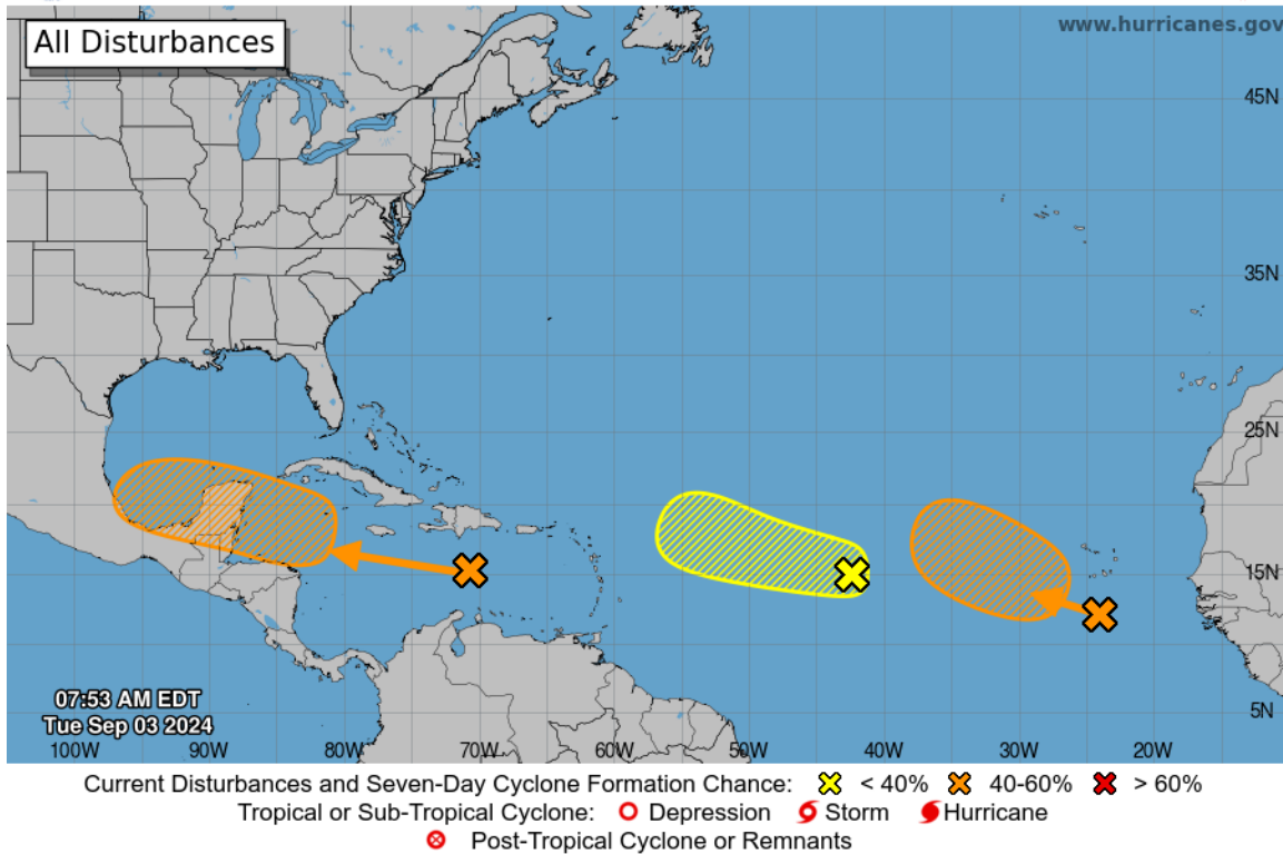
Figure 3: Current National Hurricane Center Atlantic Tropical Weather Outlook.
