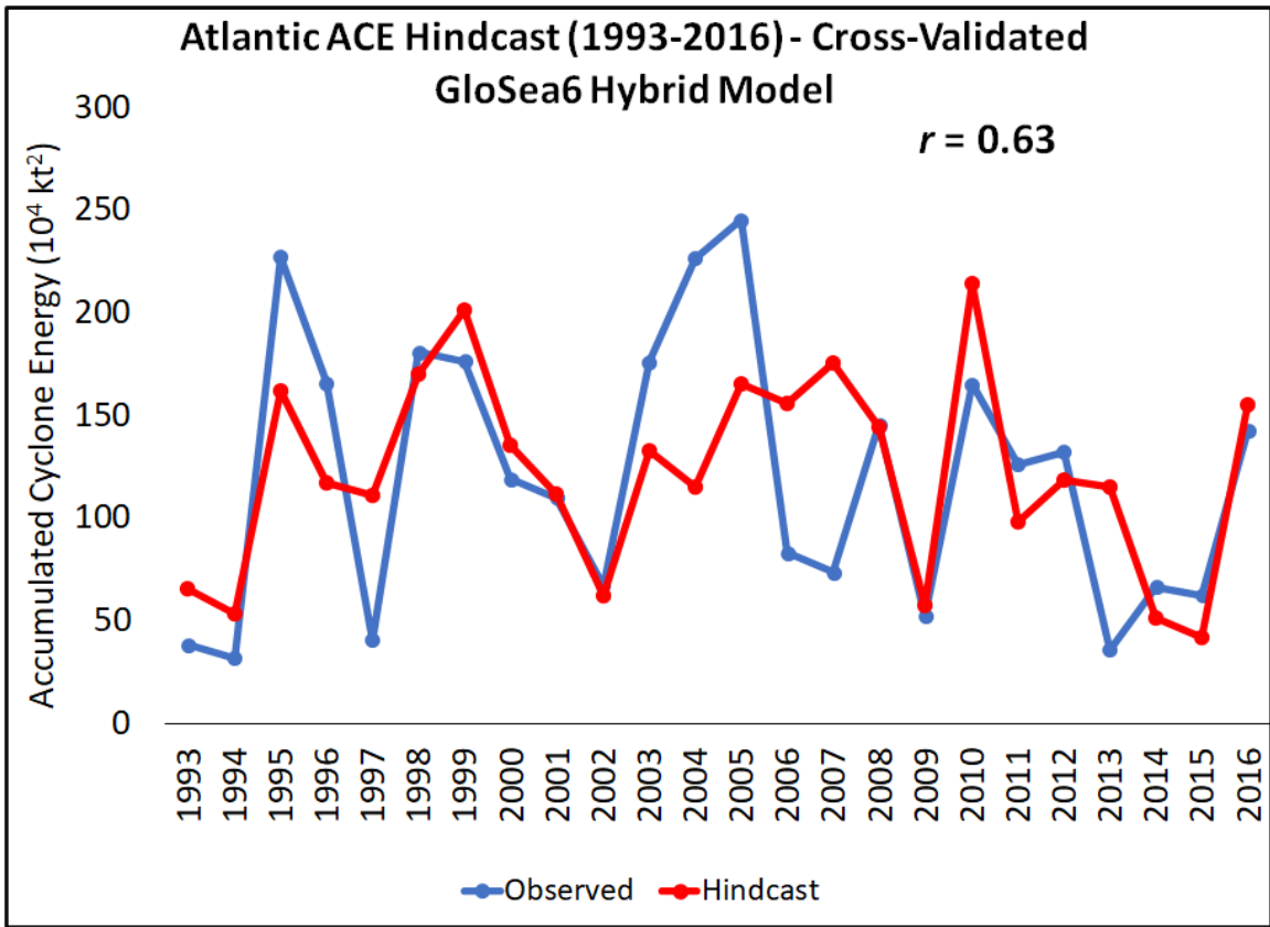
Figure 10: Observed versus May cross-validated statistical/dynamical hindcast values of ACE for 1993-2016 from GloSea6.
