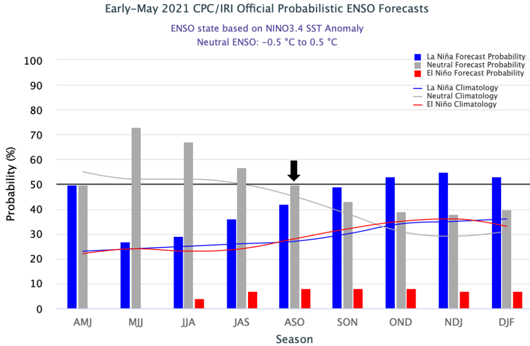
Figure 19: Official NOAA forecast for ENSO. The black arrow highlights the peak of the Atlantic hurricane season (August-October).
