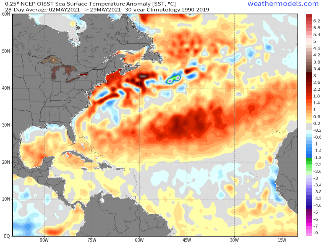
Figure 20: Recent four-week average of North Atlantic SSTs.
