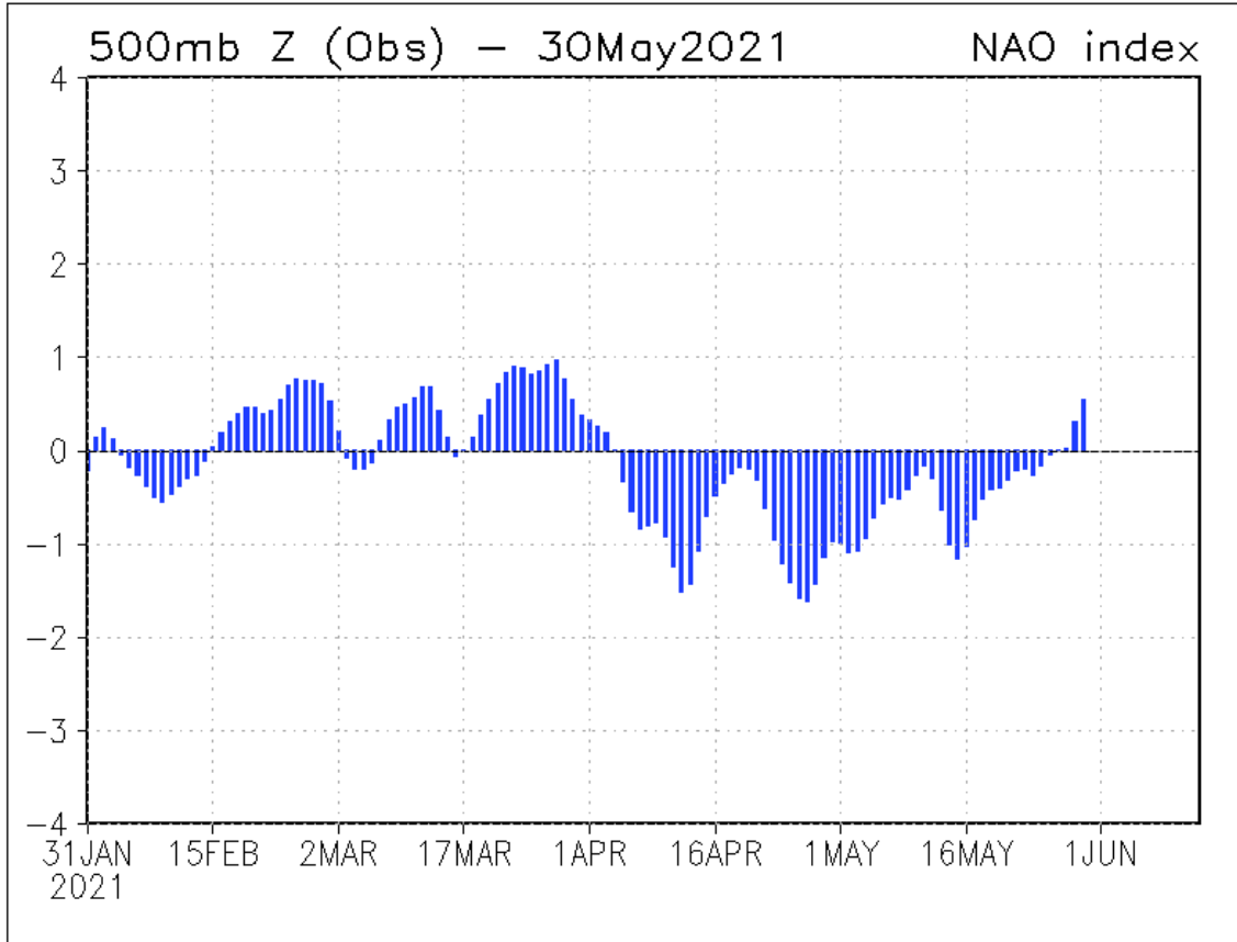
Figure 23: Observed standardized values of the daily NAO since February. The NAO was generally positive in February and March but has been predominately negative since that time.
