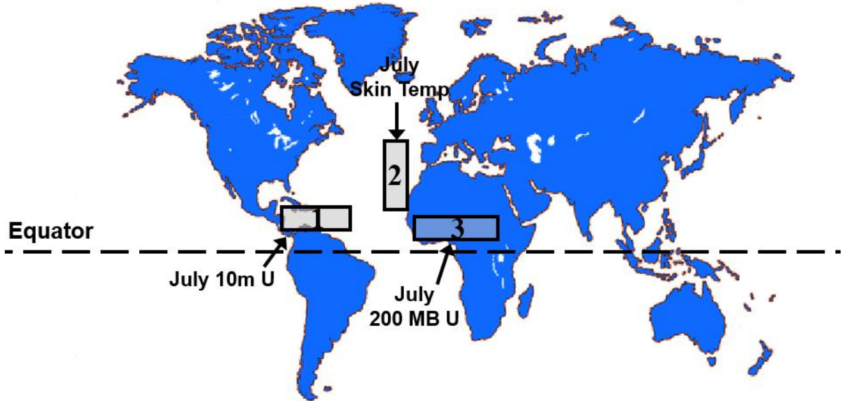
Figure 8: Location of predictors for our statistical/dynamical extended-range statistical prediction for the 2021 hurricane season. This forecast uses either the ECMWF SEAS5 model or the UK Met Office GloSea6 model to predict July conditions in the three boxes displayed and uses those predictors to forecast ACE.
