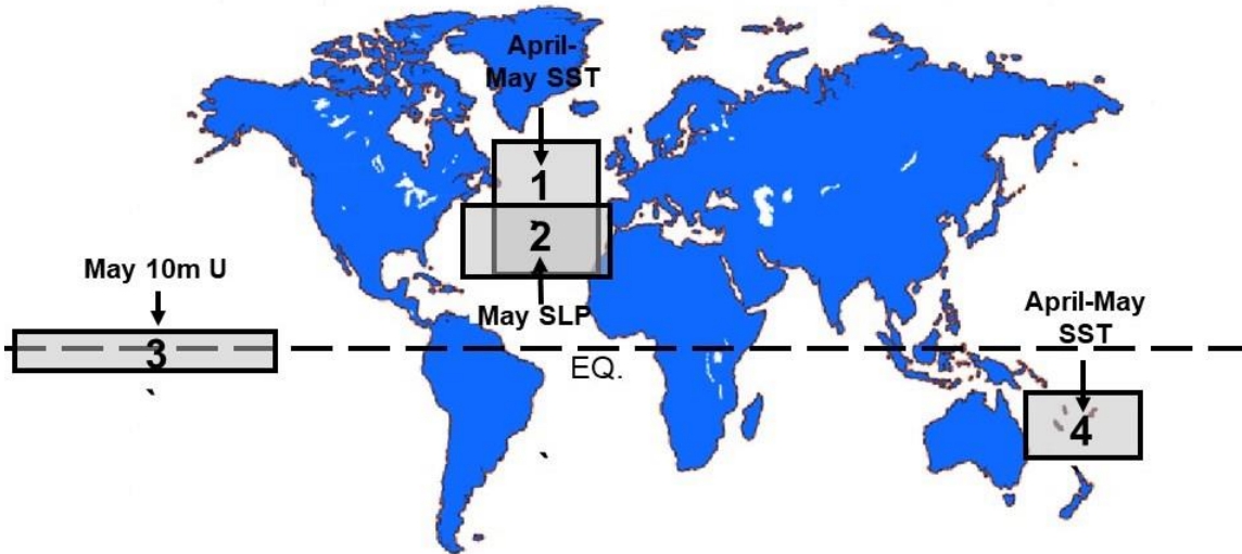
Figure 2: Location of predictors for our early June extended-range statistical prediction for the 2021 hurricane season.
