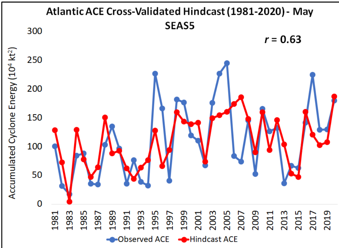
Figure 9: Observed versus May cross-validated statistical/dynamical hindcast values of ACE for 1981-2018 as well as real-time forecasts from SEAS5 for 2019-2020.
