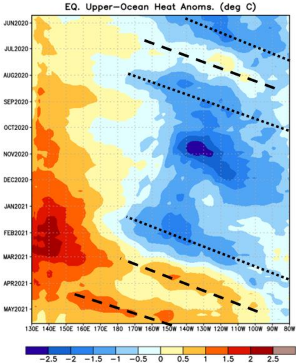
Figure 16: Upper-ocean heat content anomalies in the tropical Pacific since June 2020. Dashed lines indicate downwelling Kelvin waves, while dotted lines indicate upwelling Kelvin waves. Downwelling Kelvin waves result in upper-ocean heat content increases, while upwelling Kelvin waves result in upper-ocean heat content decreases.
