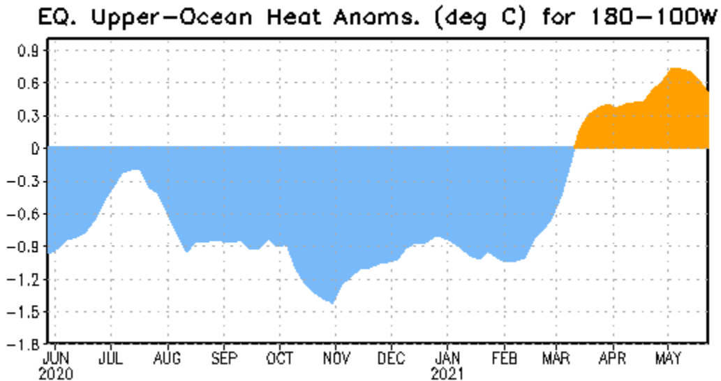
Figure 14: Central and eastern equatorial Pacific upper ocean (0-300 meters) heat content anomalies over the past year. Upper ocean heat content anomalies have increased considerably since mid-February.
