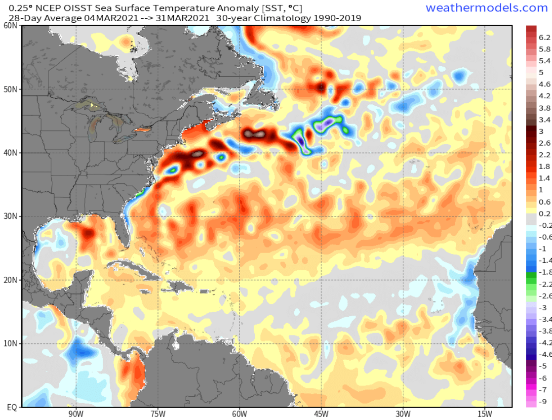
Figure 21: Four-week-averaged North Atlantic SST anomalies ending on 31 March.
