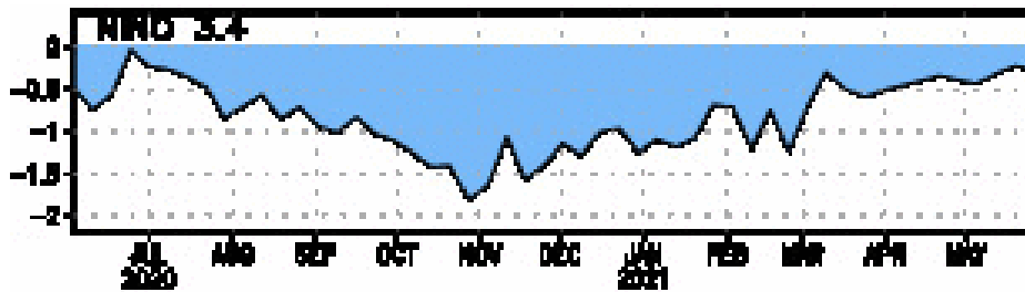
Figure 13: Nino 3.4 SST anomalies from June 2020 through May 2021. Figure courtesy of Climate Prediction Center.
