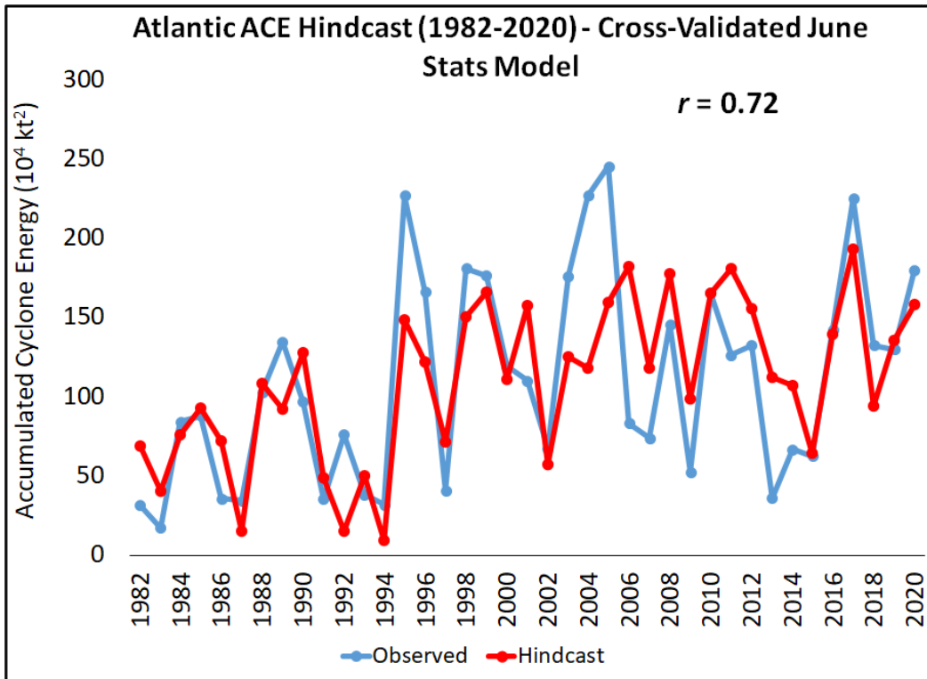
Figure 1: Observed versus early June cross-validated hindcast values of ACE for the statistical model for 1982-2020.
