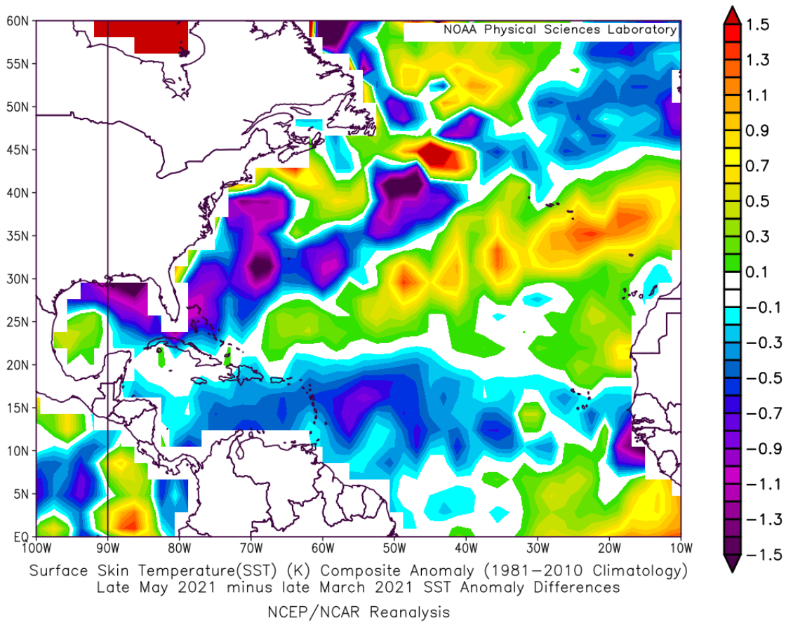
Figure 22: Late May 2021 minus late March 2021 SST anomaly changes.
