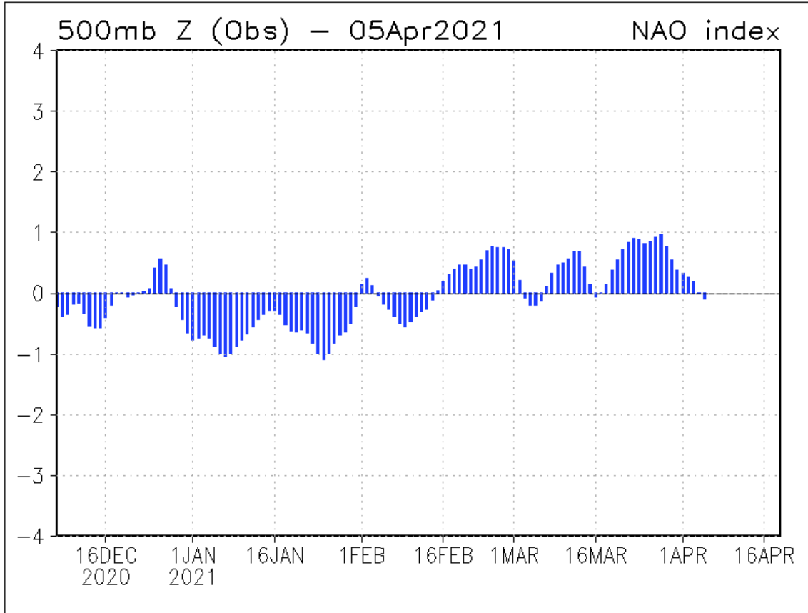
Figure 21: Observed standardized values of the daily NAO since mid-December 2020. The NAO was generally negative in January through mid-February and positive from mid-February through the end of March.
