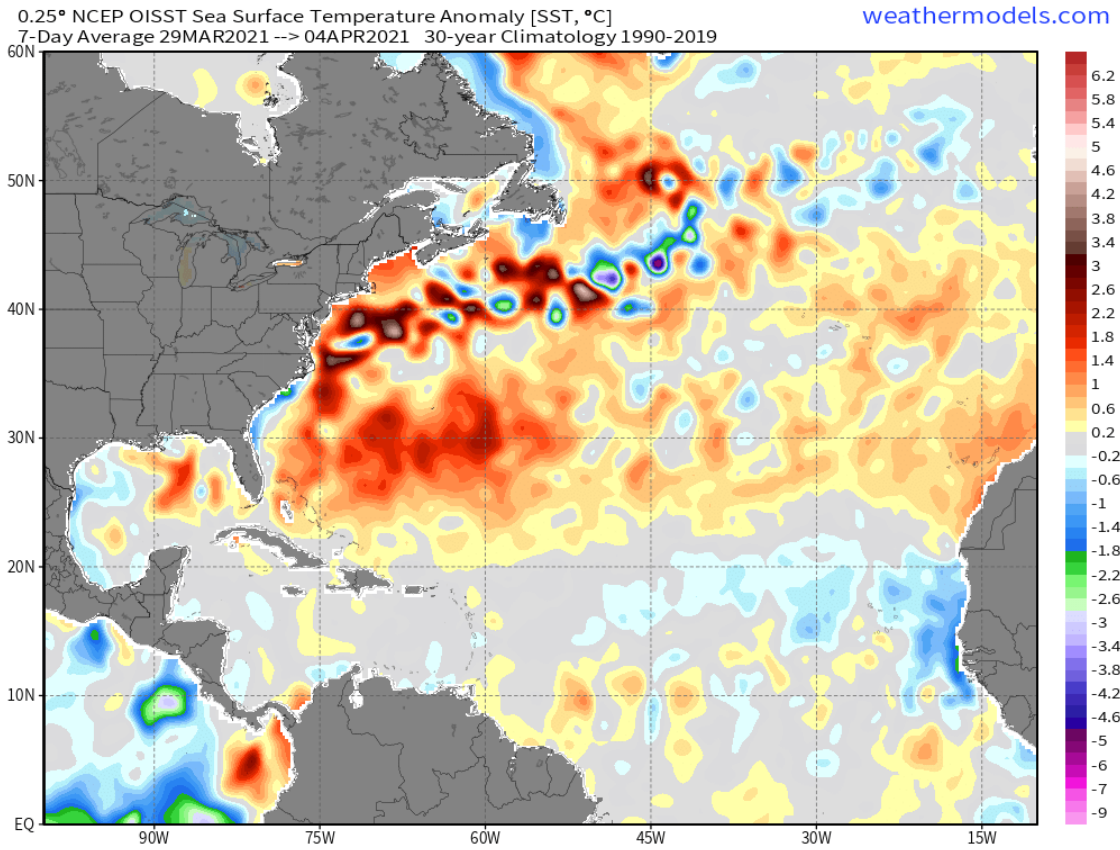
Figure 19: Late March 2021 SST anomaly pattern across the Atlantic Ocean.
