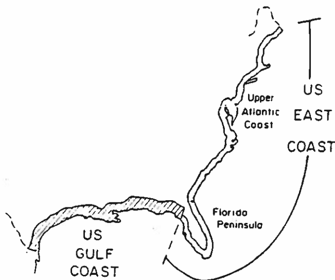
Figure 4: Portrayal of the separation of the two basic U.S. coastal areas which have different climate associations with their landfalling major hurricanes.
