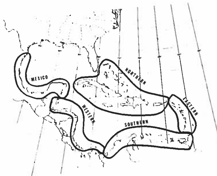
Figure 6: Caribbean Basin areas for which the probability of hurricanes and major hurricane passage through these areas are specified in Table 13.
